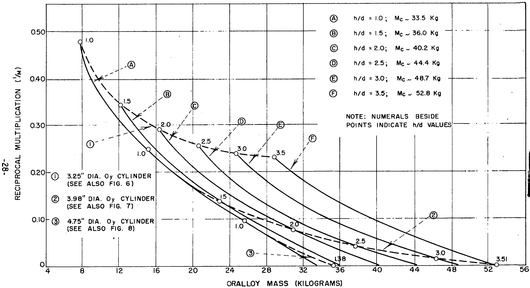
FIG. 16 CRITICAL MASS DETERMINATIONS FOR ORALLOY CYLINDERS WITH CONSTANT h/d RATIOS IN 1.12" THICK TUBALLOY TAMPERS ( h/d > 1.0 )
