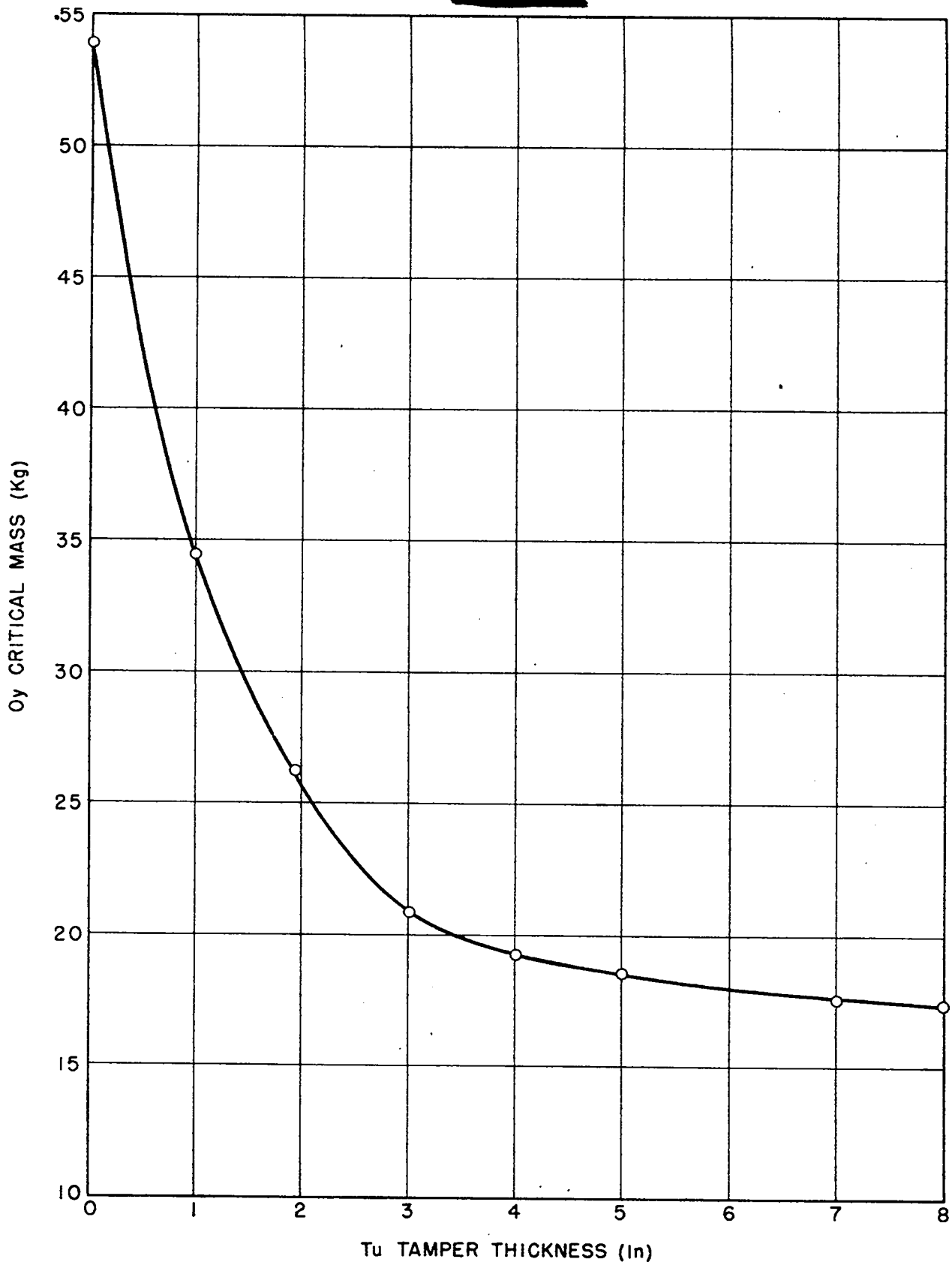
FIG. 15 Oγ CRITICAL MASS VS Tu TAMPER THICKNESS FOR SPHERES
