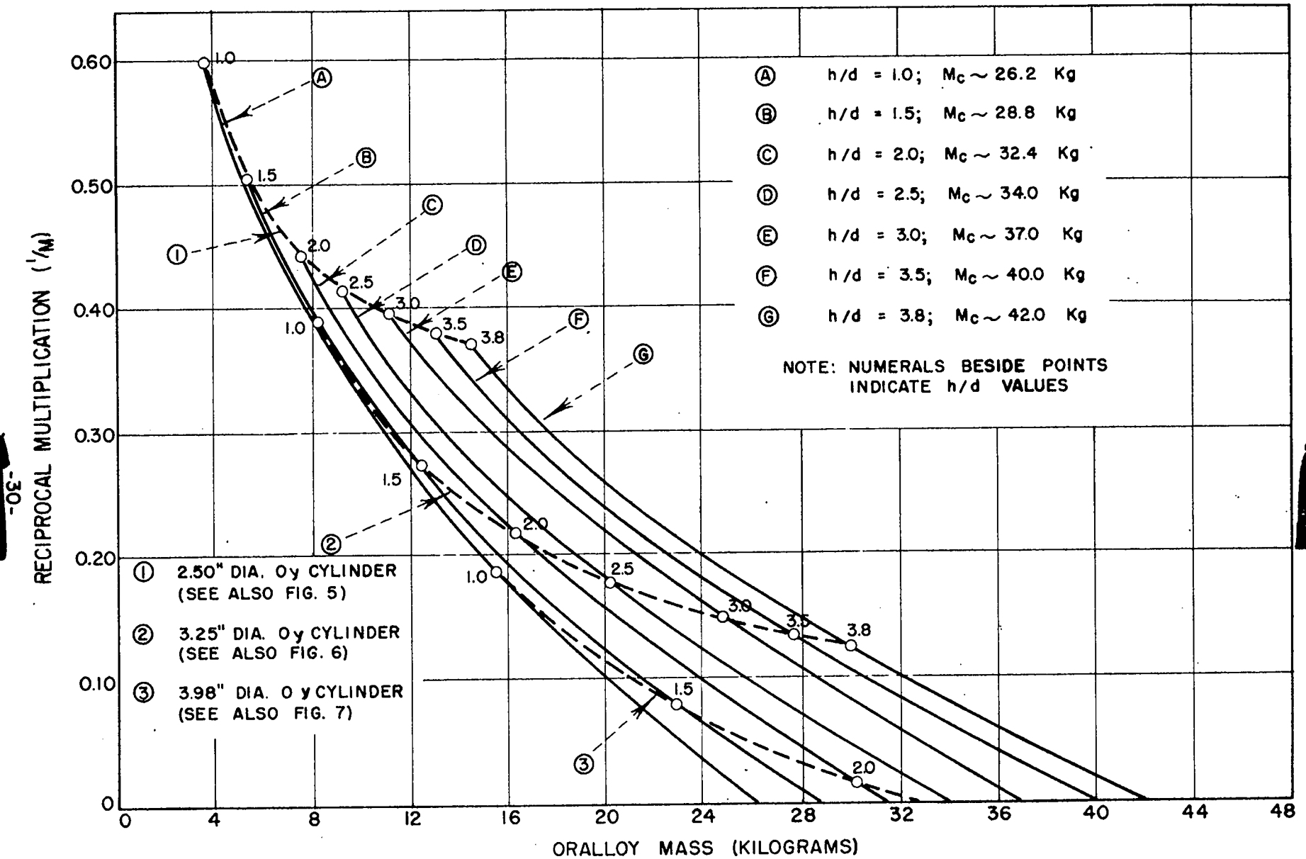
FIG. 18 CRITICAL MASS DETERMINATIONS FOR ORALLOY CYLINDERS WITH CONSTANT h/d RATIOS IN 1.87" THICK TUBALLOY TAMPER
