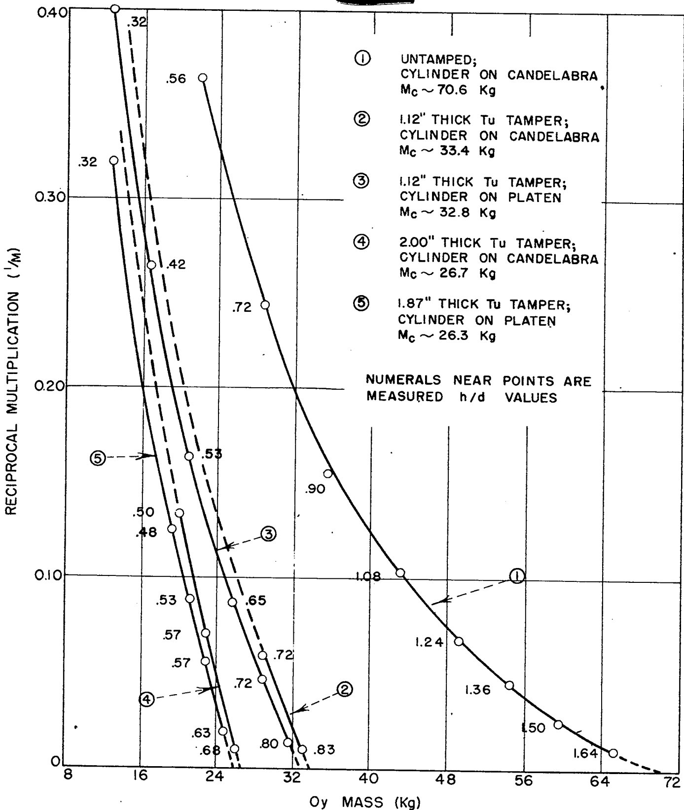
FIG. 9 RECIPROCAL MULTIPLICATION MEASUREMENTS ON 5.50" DIAMETER O_y CYLINDERS
