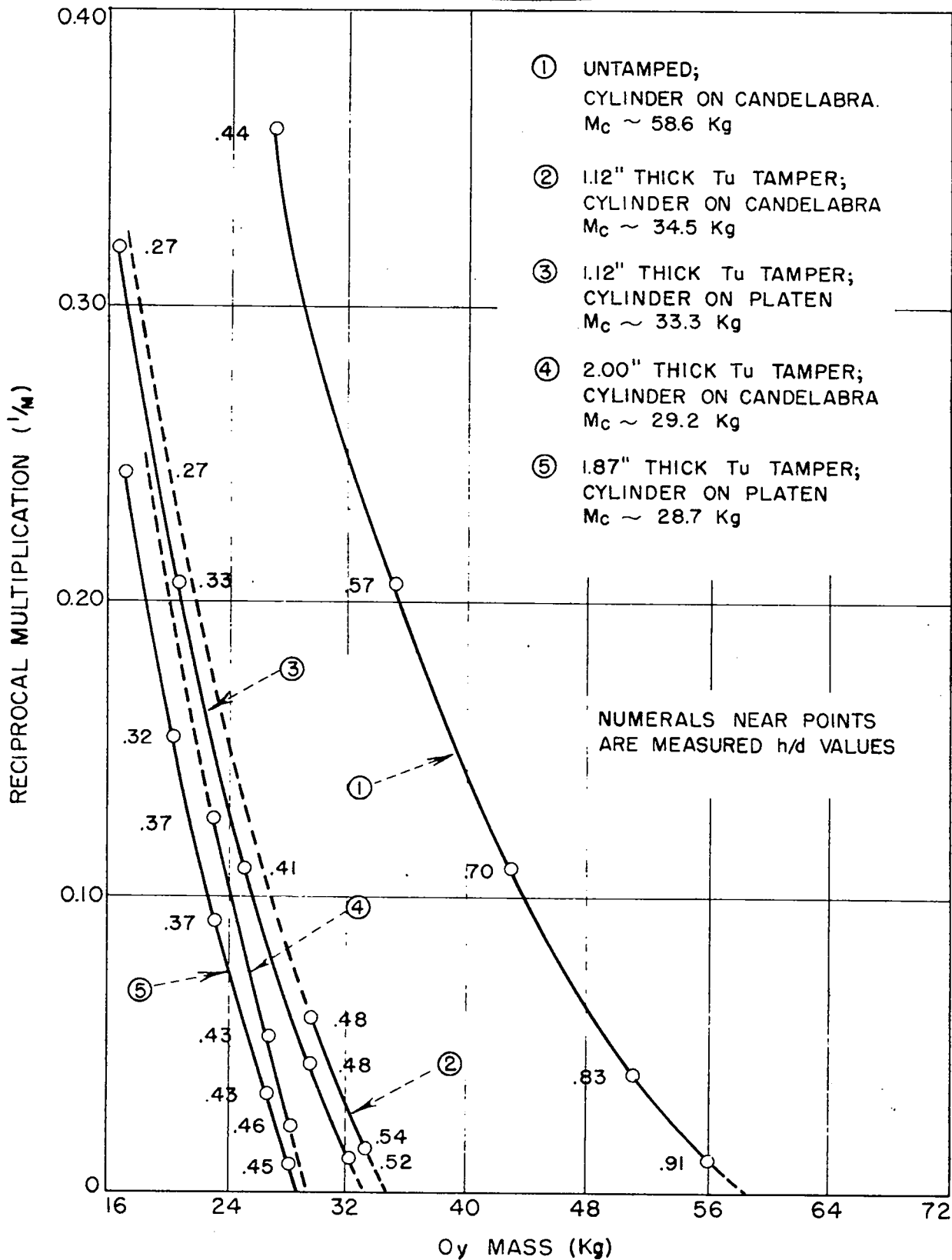
FIG. 10 RECIPROCAL MULTIPLICATION MEASUREMENTS ON 6.37" DIAMETER O_y CYLINDERS
