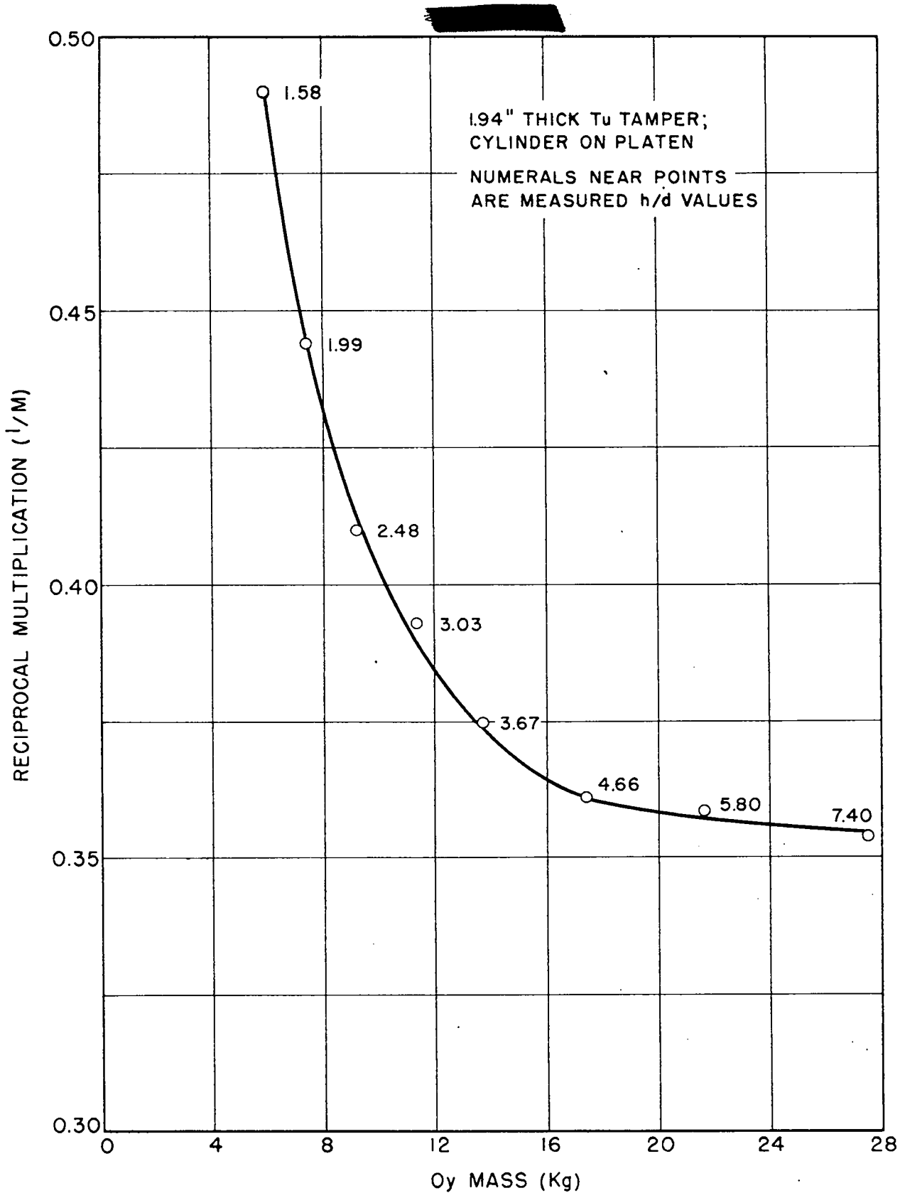
FIG. 5 RECIPROCAL MULTIPLICATION MEASUREMENTS ON 2.50" DIAMETER Oy CYLINDER
