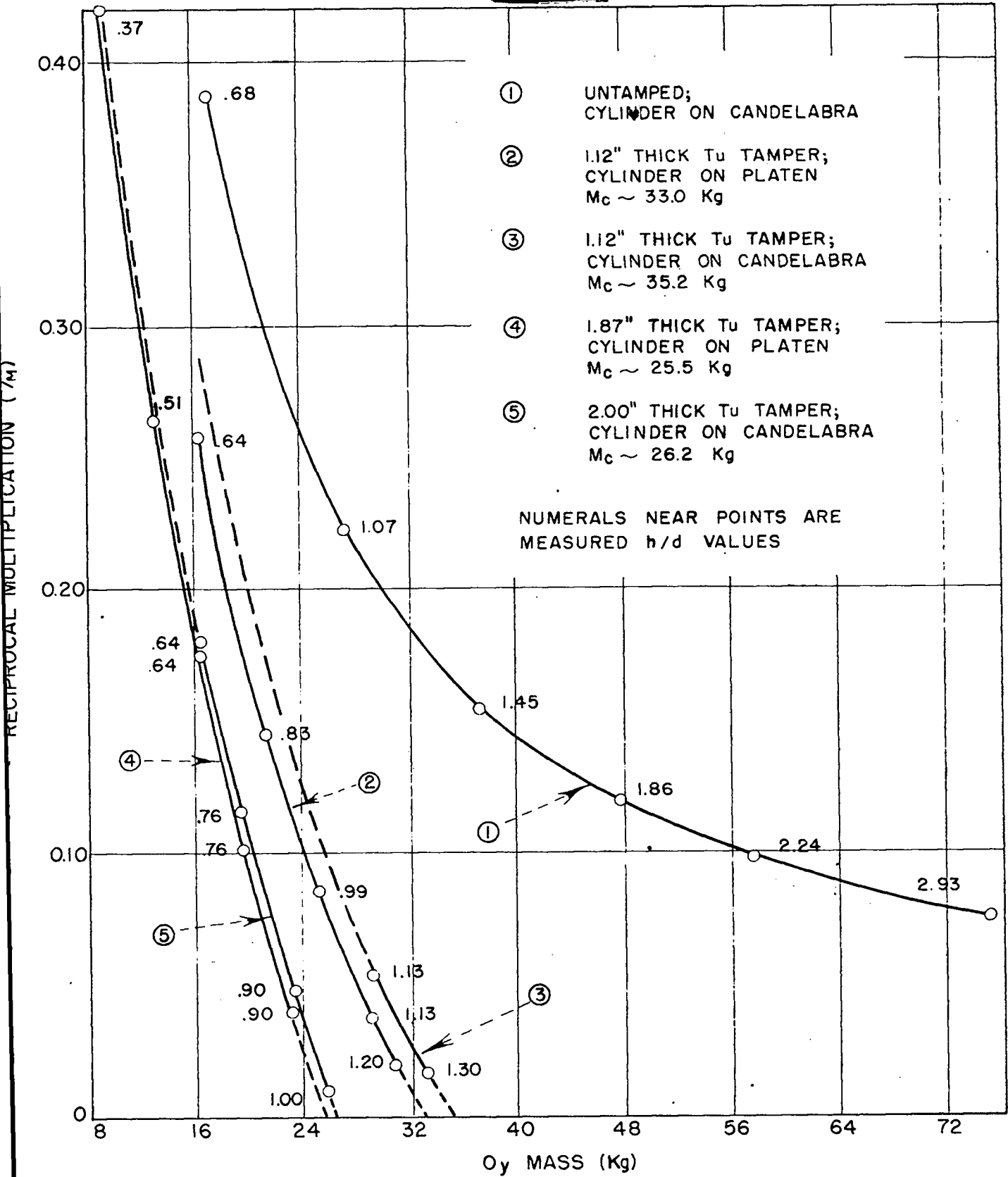
FIG. 8 RECIPROCAL MULTIPLICATION MEASUREMENTS ON 4.75" DIAMETER Oy CYLINDERS
