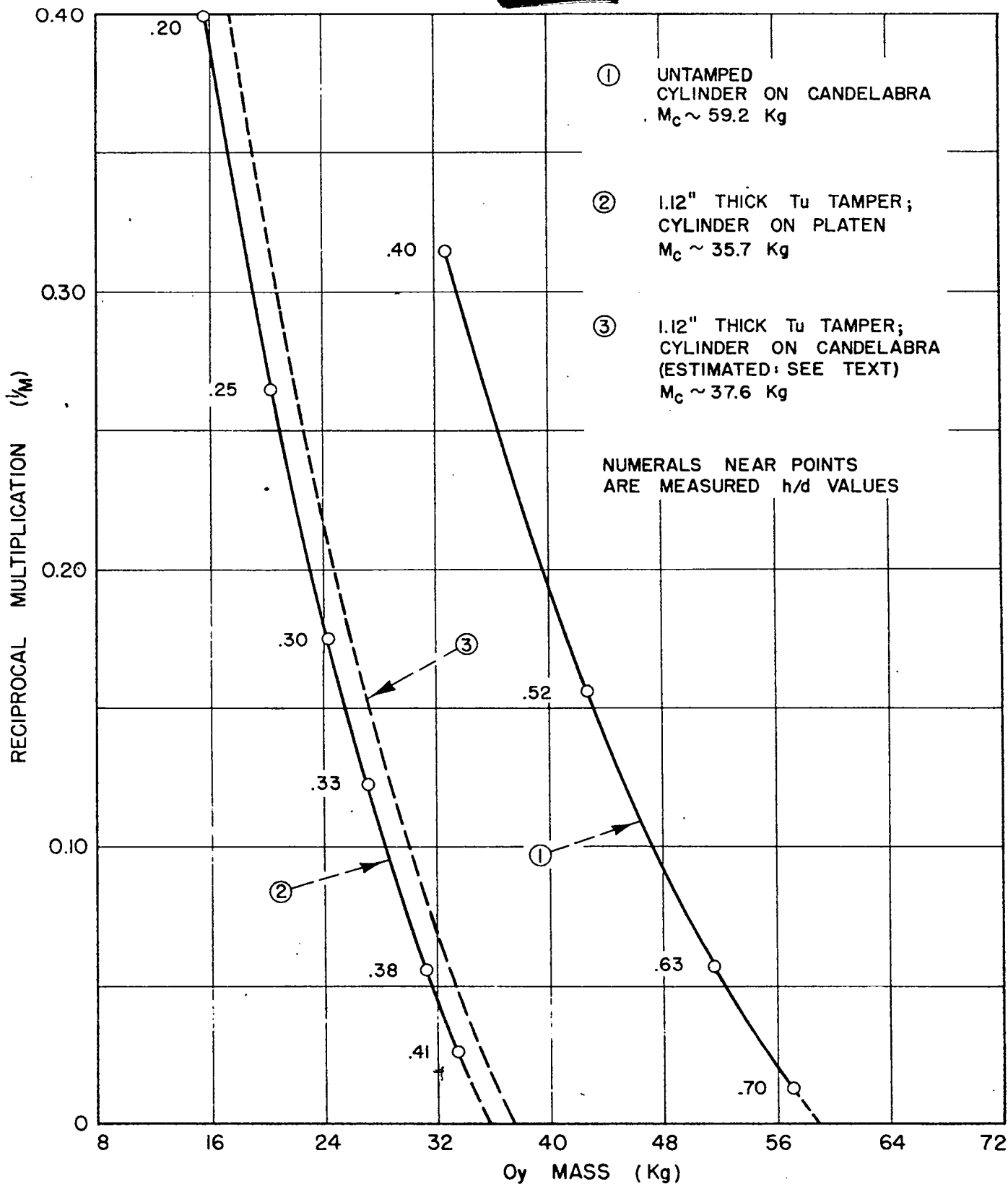
FIG. II RECIPROCAL MULTIPLICATION MEASUREMENTS ON 7.00" DIAMETER O_y CYLINDERS
