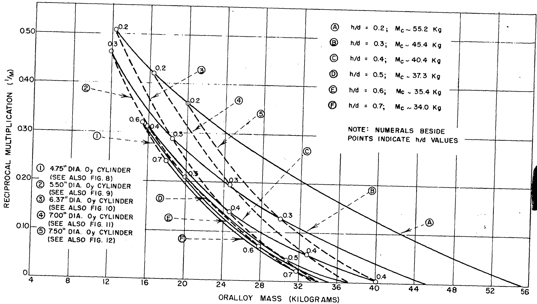
FIG. 17 CRITICAL MASS DETERMINATIONS FOR ORALLOY CYLINDERS WITH CONSTANT h/d RATIOS IN 1.12" THICK TUBALLOY TAMPERS
