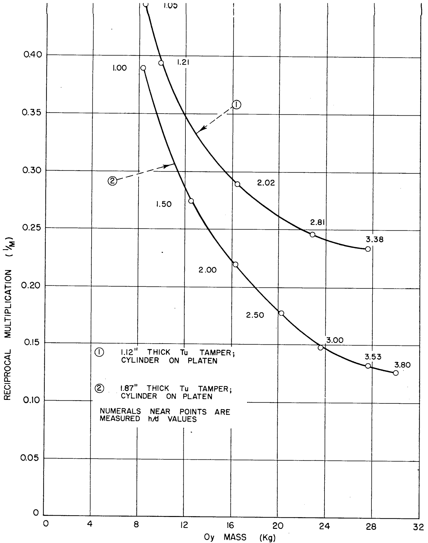
FIG. 6 RECIPROCAL MULTIPLICATION MEASUREMENTS ON 3.25" DIAMETER Oy CYLINDERS
