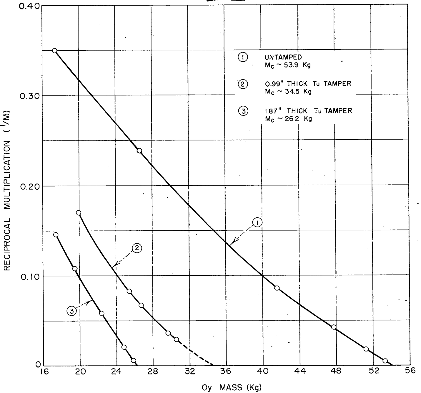
FIG. 14 RECIPROCAL MULTIPLICATION MEASUREMENTS ON Oy PSEUDOSPHERES
