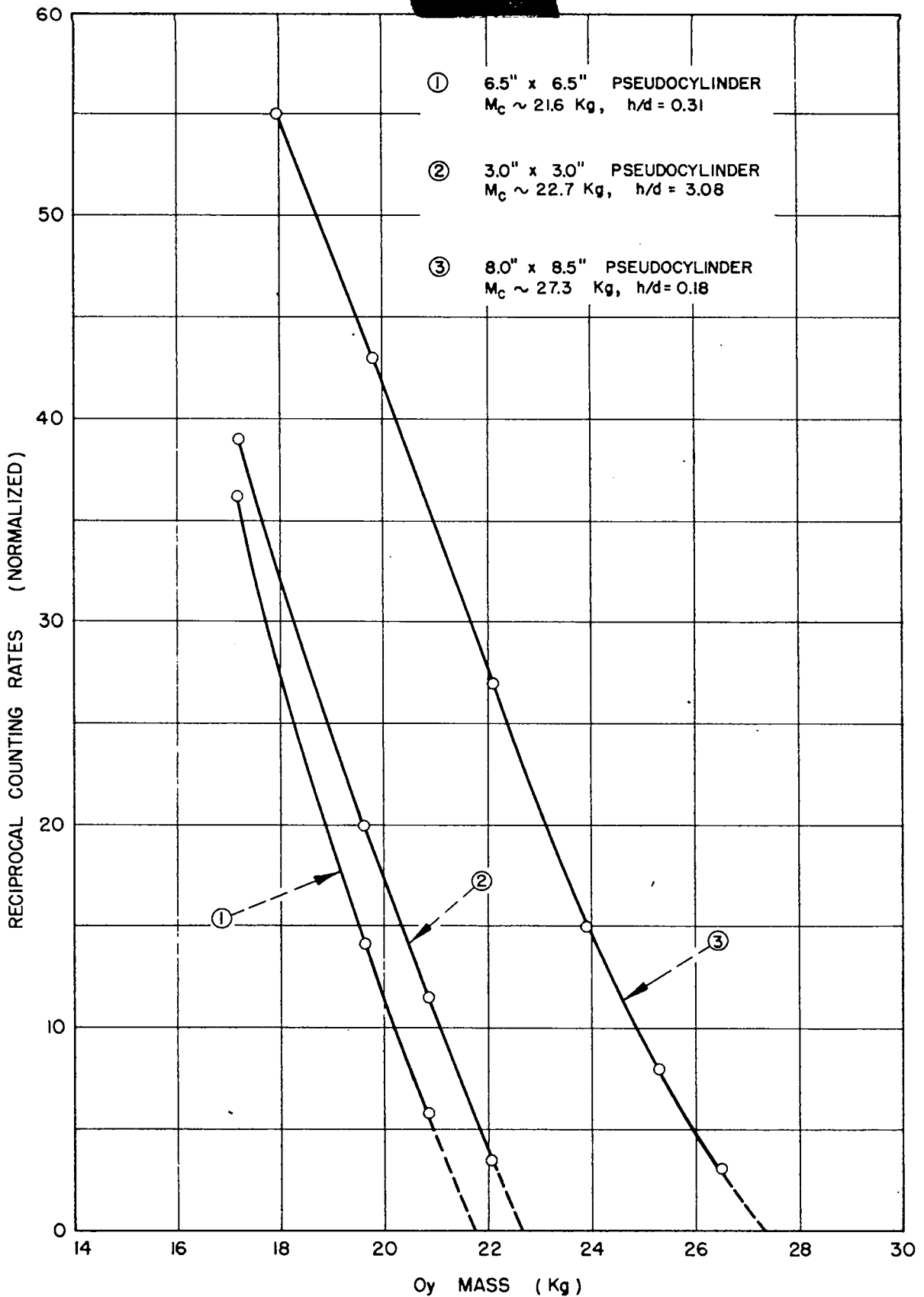
FIG. 13 RECIPROCAL COUNTING RATE MEASUREMENTS ON Oy PSEUDOCYLINDERS IN 8.0" THICK Tu TAMPER
